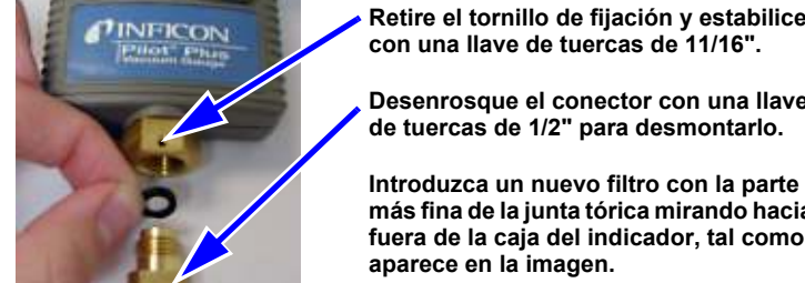
Figura 2. Conector del Pilot Plus
